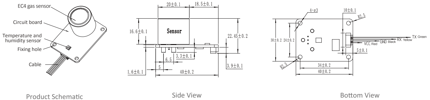
4Pin cable size diagram
